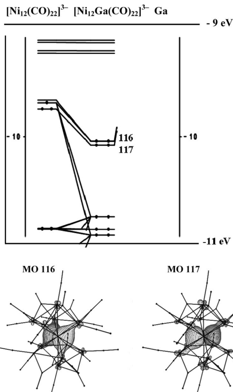
Figure 5. Frontier region of the EHMO diagram (top) calculated with CACAO [14] and picture of the quasidegenerate 116 and 117 HOMOs of [\text{Ni}_{12}\text{Ga}(\text{CO})_{22}]^{3-} (bottom).
